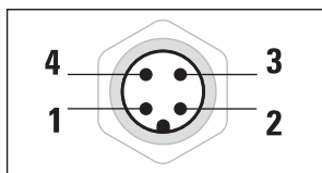
Schematic drawing of M12 plug
