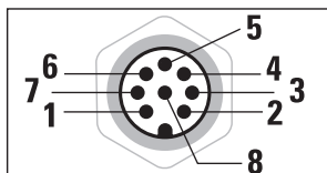
Schematic drawing of M12 plug
