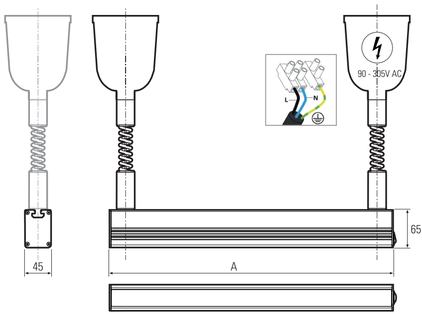
PROFILED AC Zuggpendel
